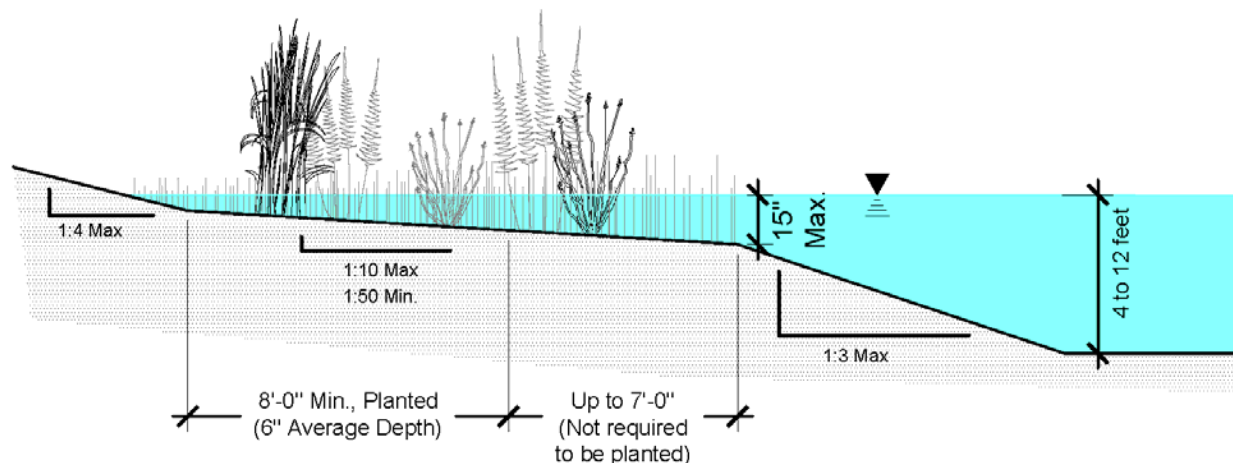
Figure 3-3. Schematic of a Submerged Bench with Plantings
